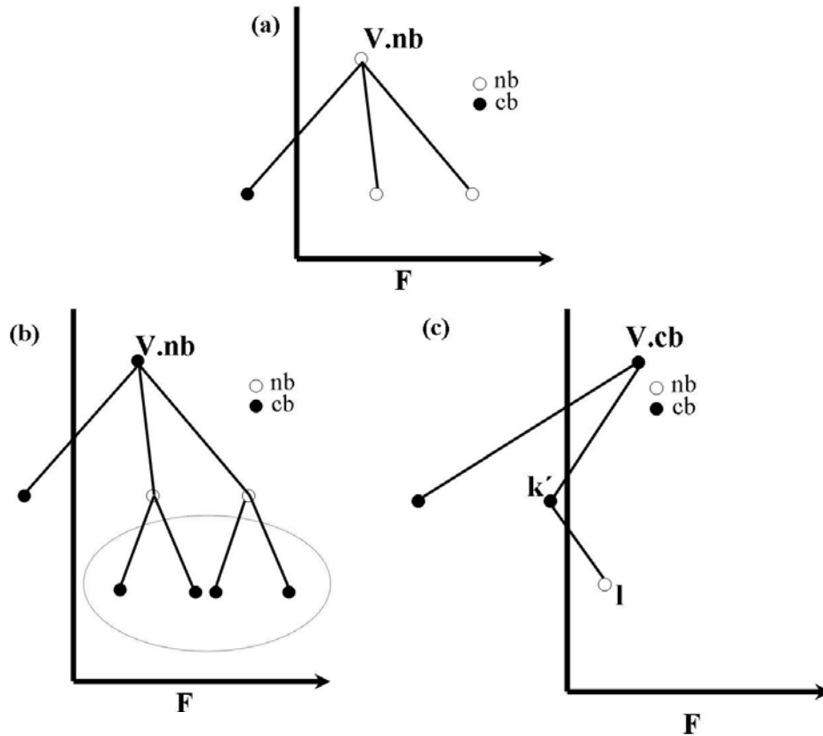
Fig. 1. Application of the algorithm dividing a TGTS into Topic and Focus
